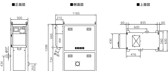
CA-100/寸法図(mm)
