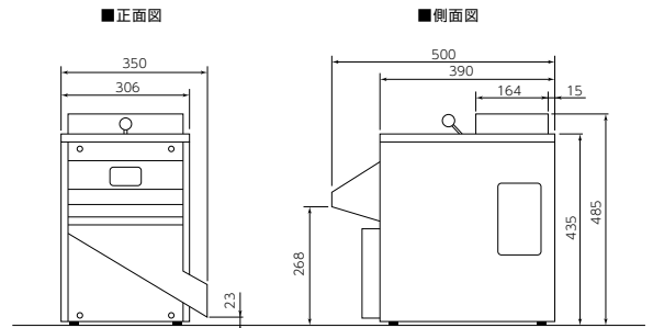
KS-1D/寸法図(mm)
