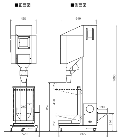
HK40A/寸法図(mm)
